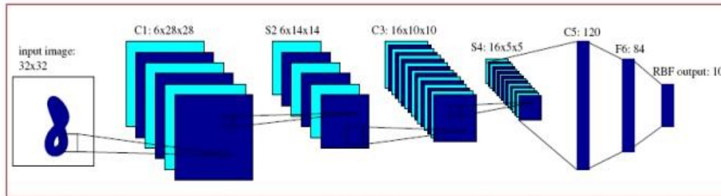
Fig 2 Convolutional Neural Network
